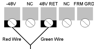
Figure A.1 Power Supply Connection
